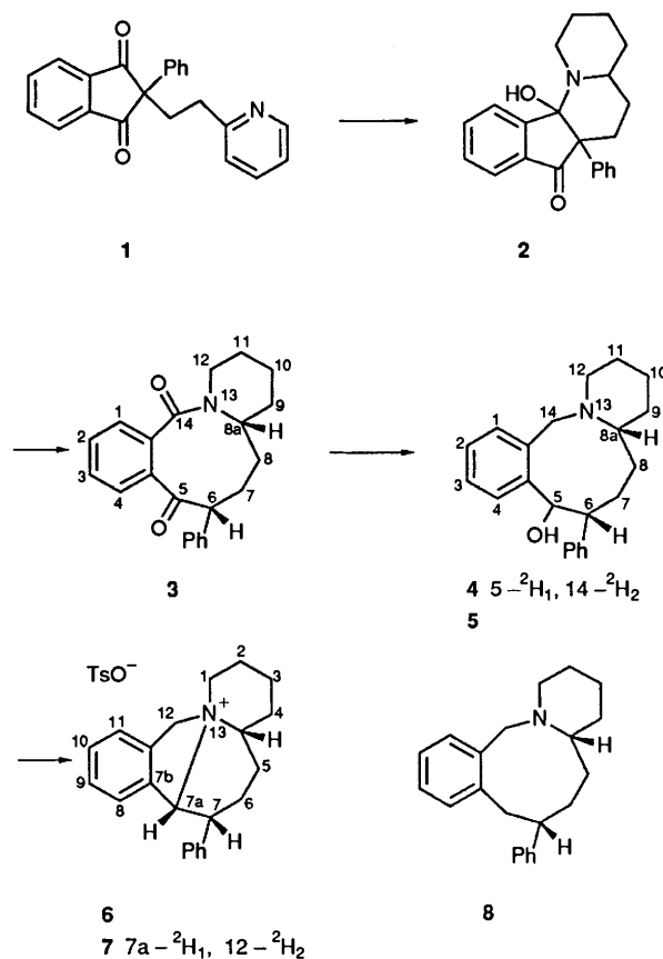
Scheme 1. Synthesis of 1,2,3,4,4 a ,5,6,7,7 a ,12-decahydro-7-phenylisoindolo[1,2- d ]quinolizin-13-ium tosylate.
